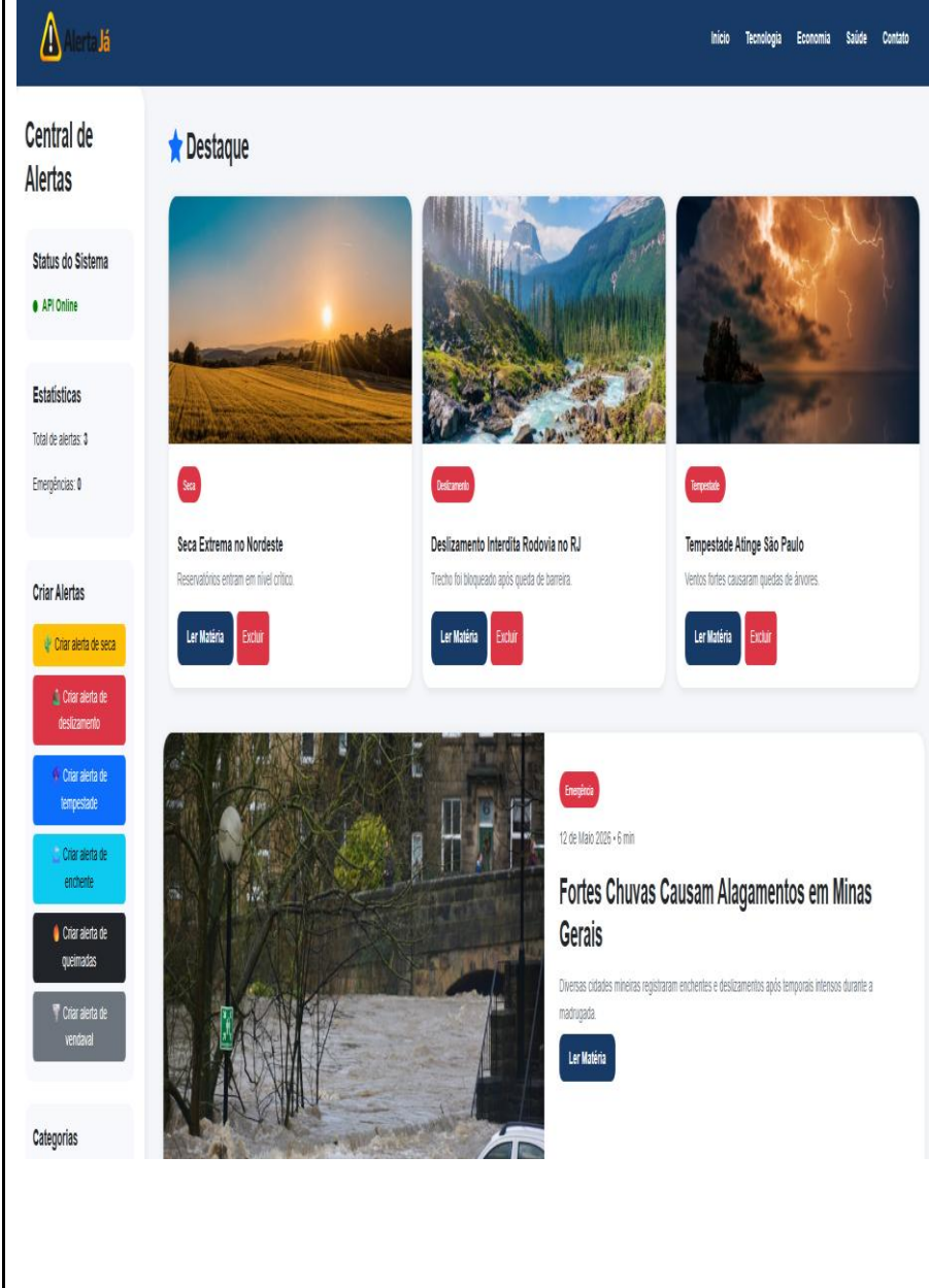
Figura 1 – Tela principal
